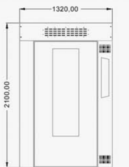
ROTORCOOK R5 .....
